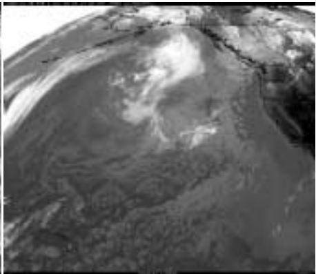
b) IR window, 10.7 \mu\text{m}
