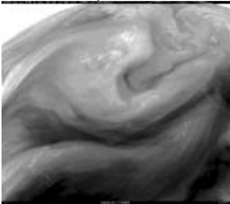
c) IR water vapor band, 6.7 \mu\text{m}
