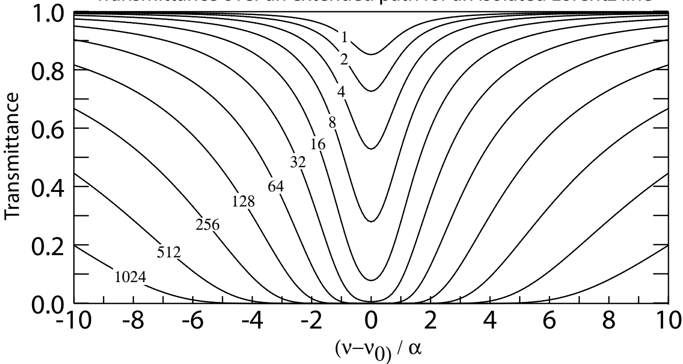
Transmittance over an extended path for an isolated Lorentz line
