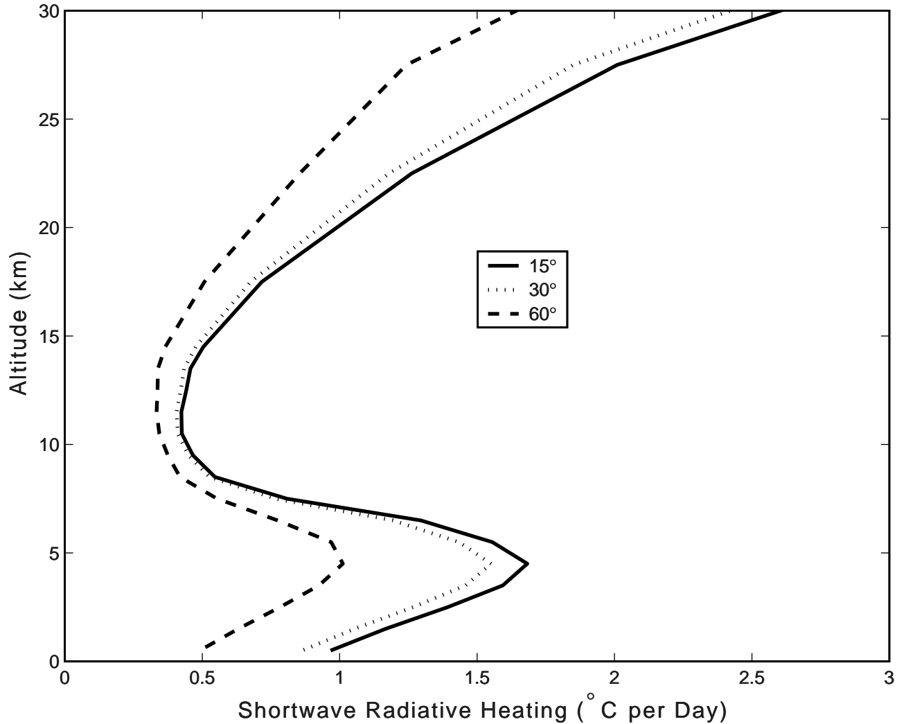
Tropical conditions with varying solar zenith angle
