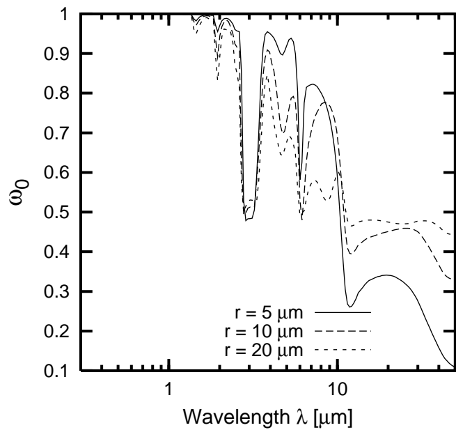
(c) Single Scatter Albedo - Cloud Droplets
