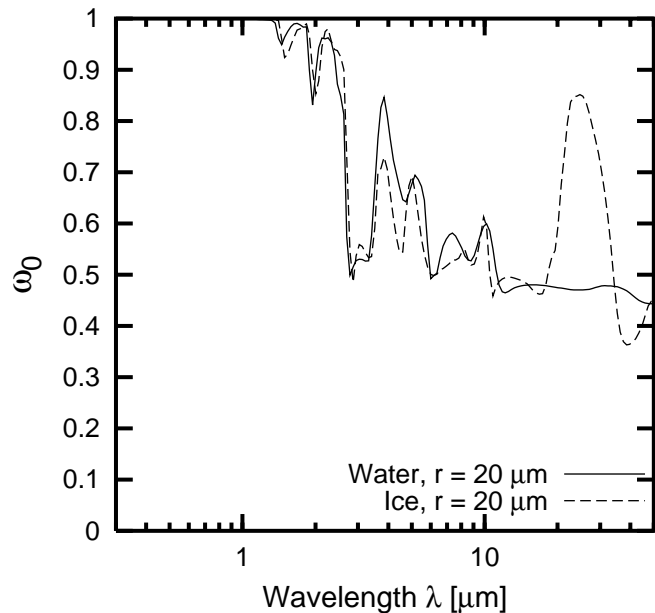
(c) Single Scatter Albedo - Cloud Droplets
