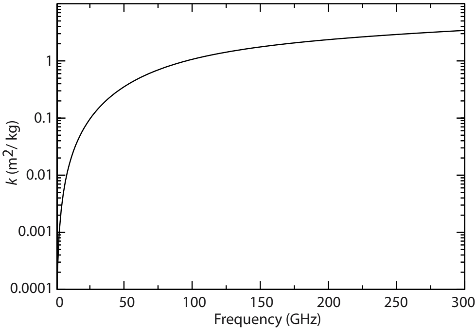
Mass absorption coefficient for cloud water
