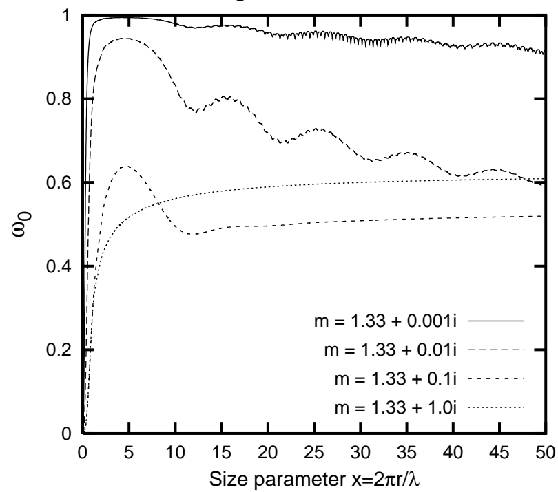
Single Scatter Albedo
