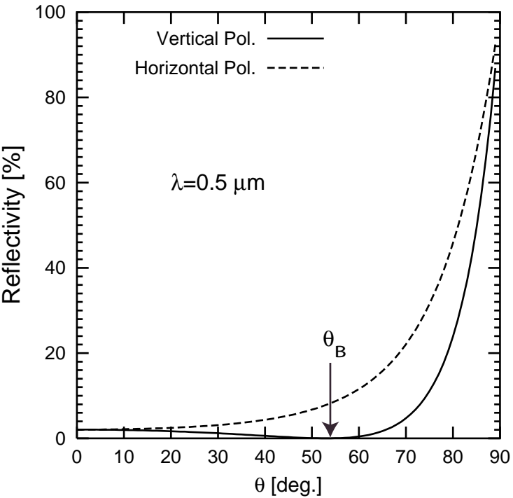
(a) Reflectivity of Water (Visible)
