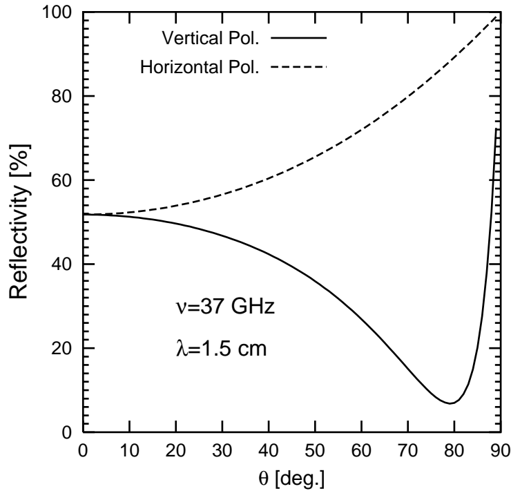
(b) Reflectivity of Water (Microwave)
