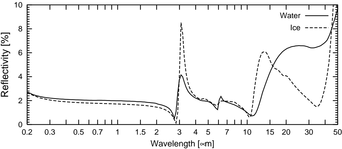
Reflectivity (Normal Incidence) of Water and Ice
