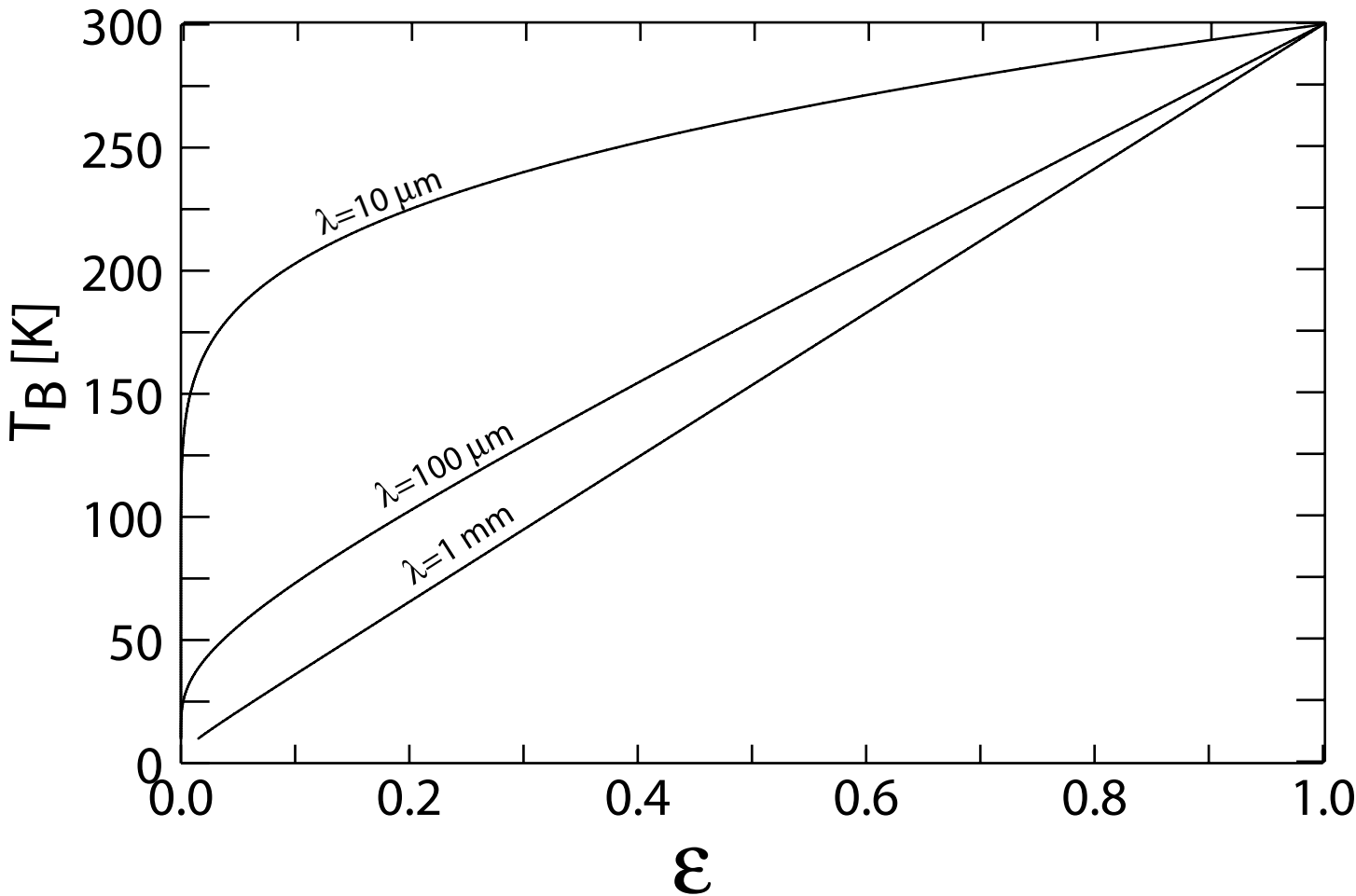
Brightness Temperature vs. Emissivity for Surface with T = 300 K
